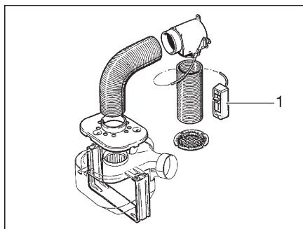
Afb. 114 Airmix-comfortpakket
