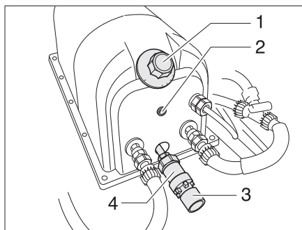
Afb. 129 Boiler Reich
