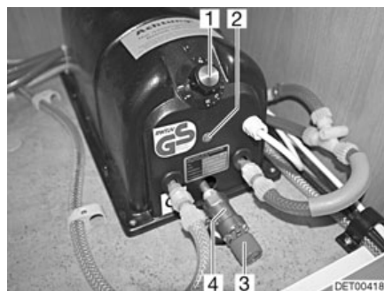
Afb. 137 Boiler Reich
